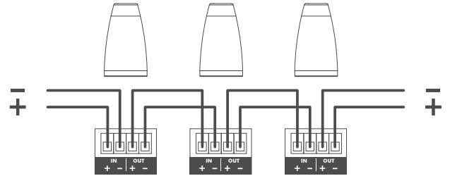
FIGURE 18: LOOP THROUGH CONNECTION
