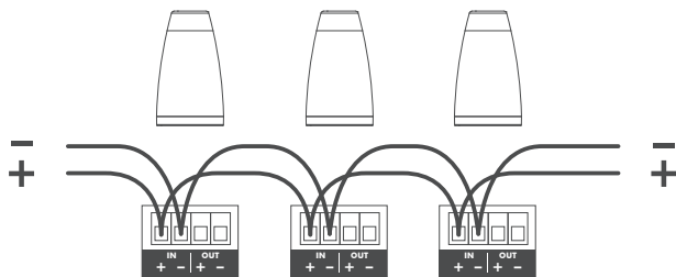
FIGURE 17: PARALLEL CONNECTION
